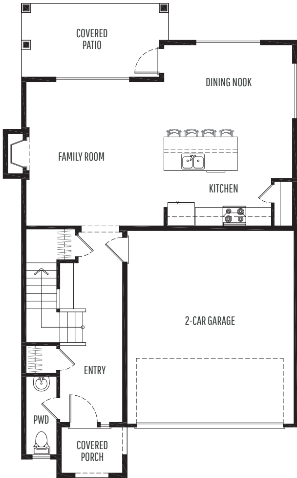
MAIN LEVEL
