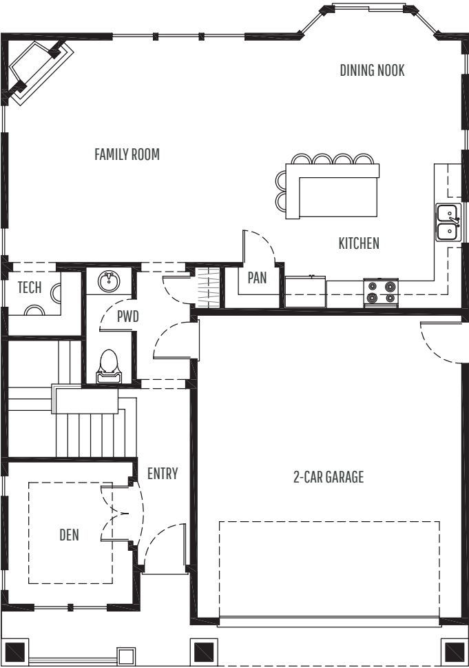
MAIN LEVEL
