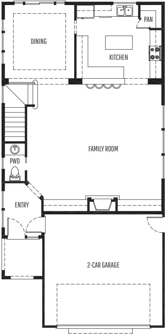
MAIN LEVEL
