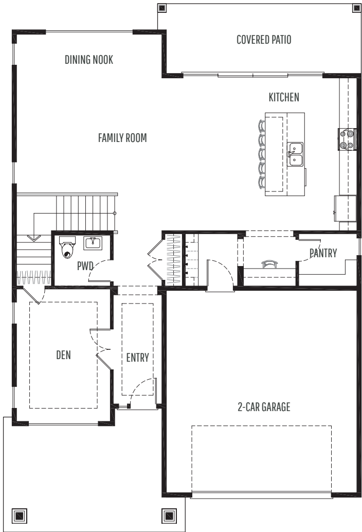
MAIN LEVEL
