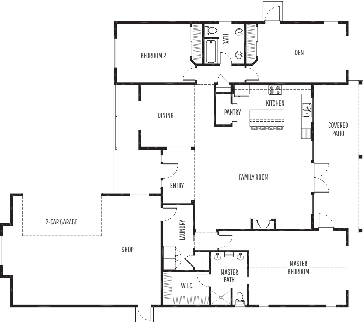
MAIN LEVEL
