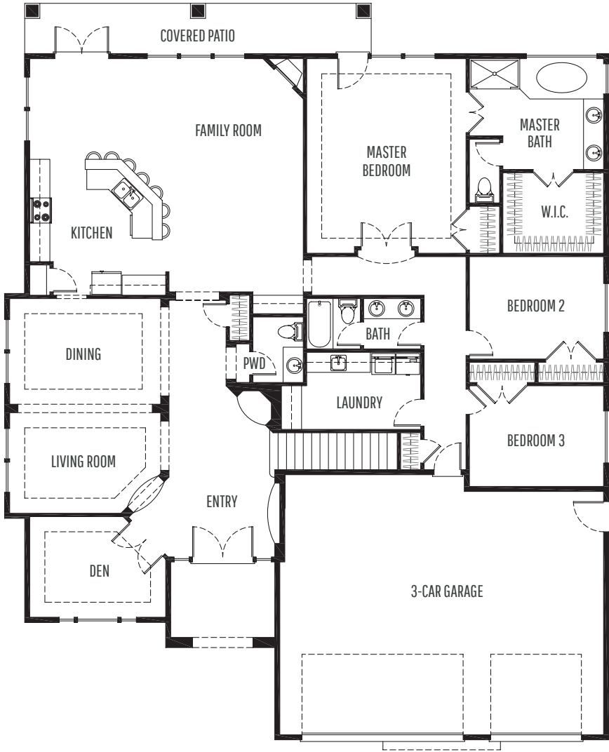
MAIN LEVEL
