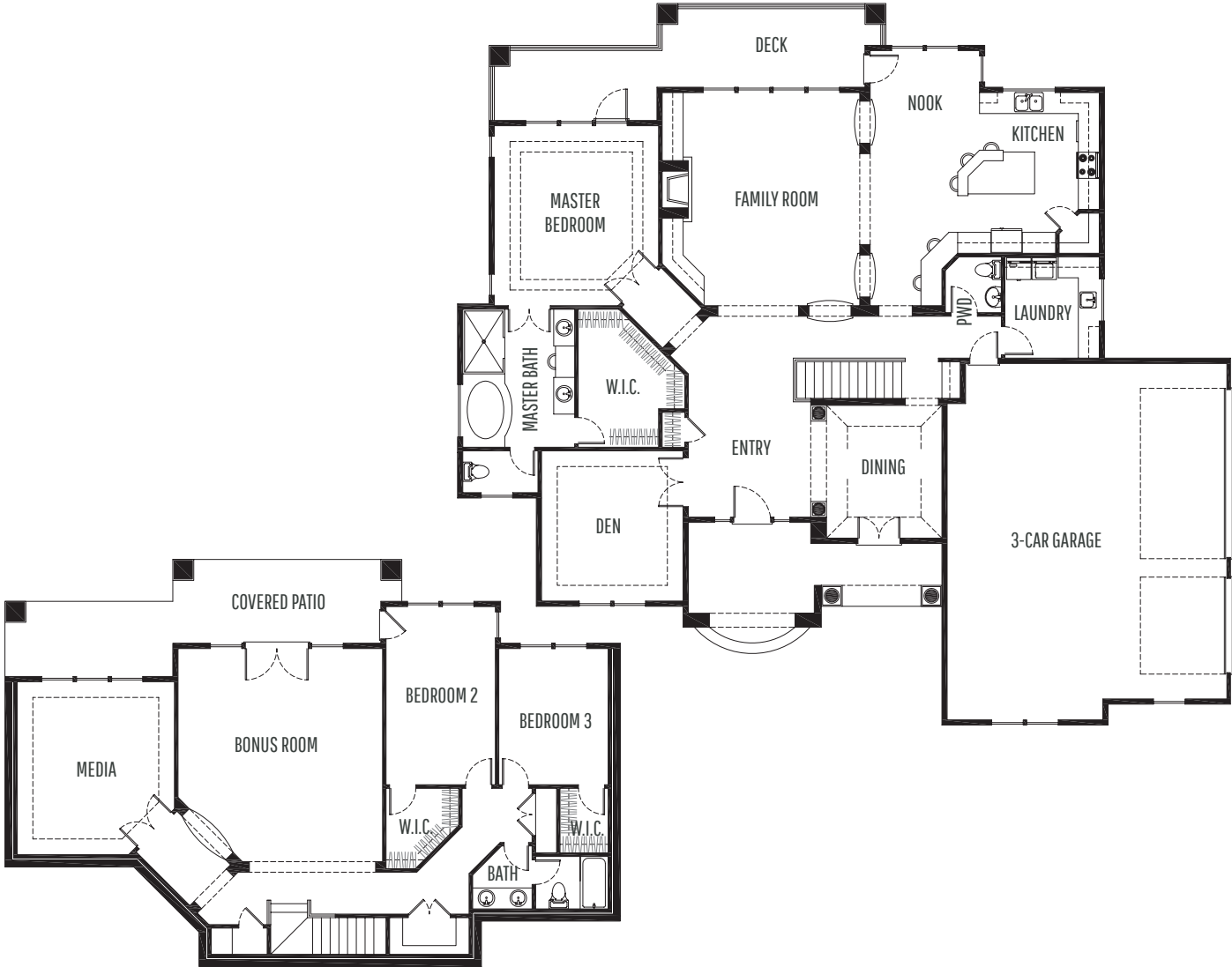
LOWER LEVEL
