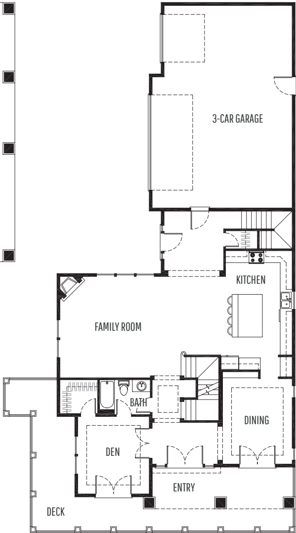
MAIN LEVEL
