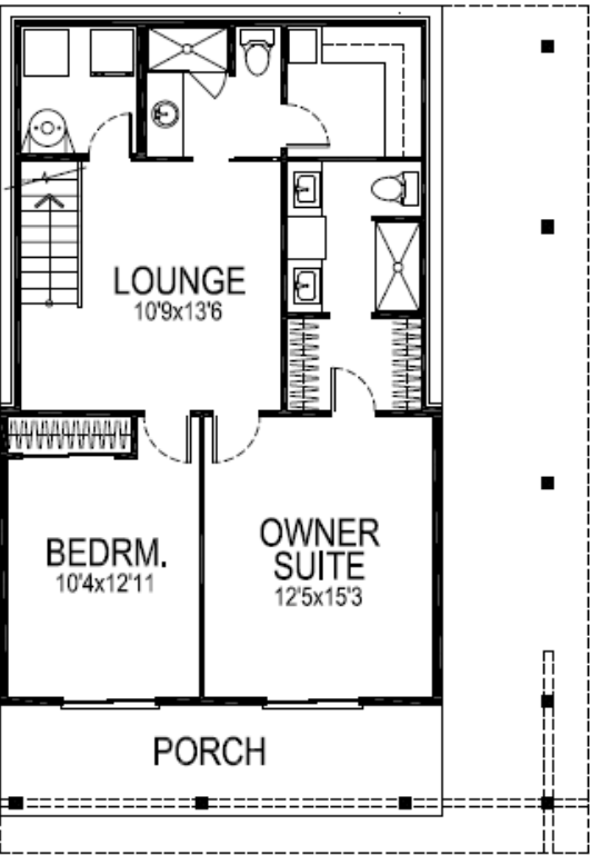
LOWER LEVEL
