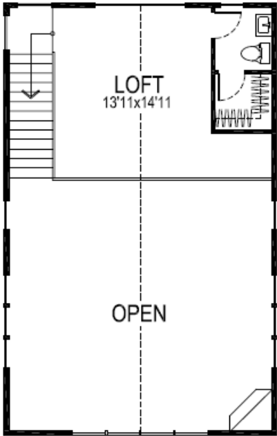
UPPER LEVEL
