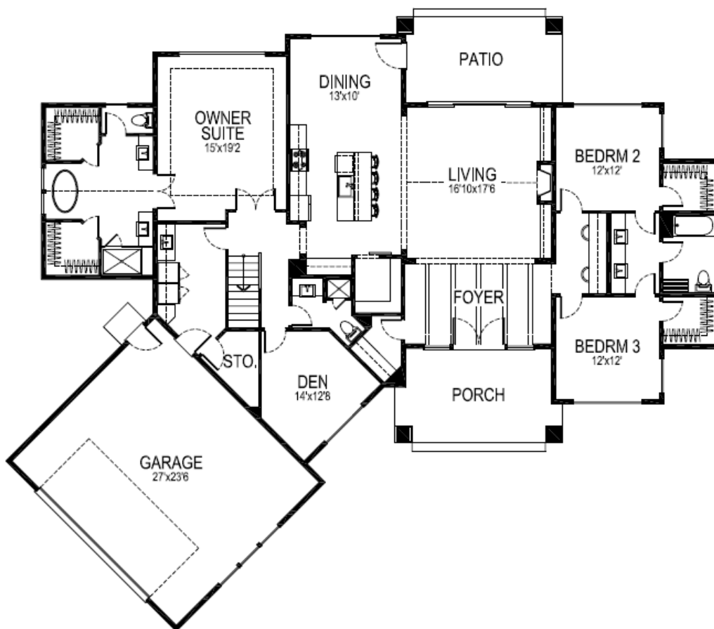
MAIN LEVEL
